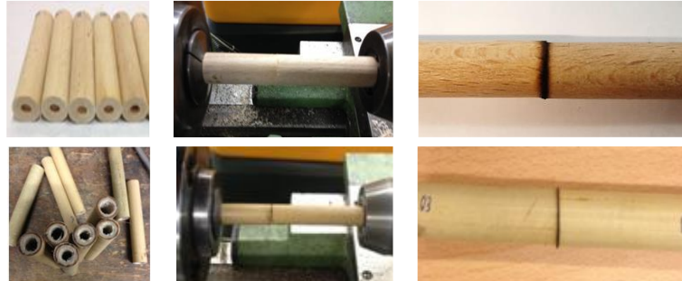
Figure 6. Friction welding on bars of wood (top) bamboo (bottom).
