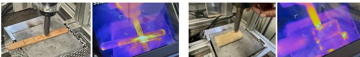
Figure 16. Principle tests for inspection task 2 (left) + 6 (right) of Tab. 1 for failure type “delamination”: test setup and result image after ultrasonic excitation - the concealed adhesive is becoming clearly apparent in the infrared image.
