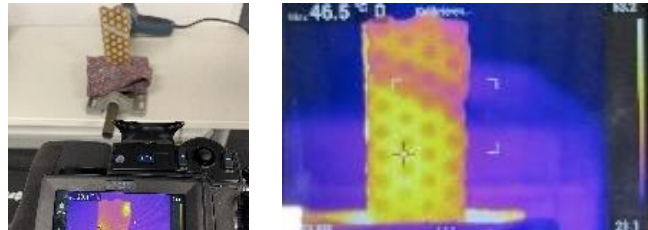
Figure 18. Principle tests for inspection task 5 of Tab. 1 for failure type “delamination”: test setup and result image after hot air excitation – the delamination in the wood top layer is becoming clearly apparent in the infrared image.
