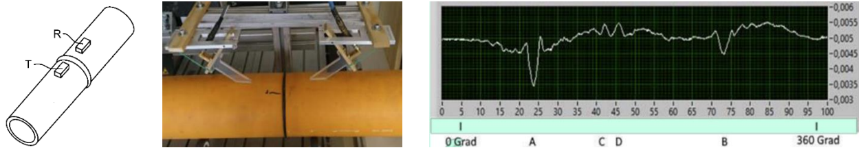
Figure 14. : Test setup pitch-catch method with positions of microwave couplers for transmitting (T) and receiving (R) (left), device under test for butt-welded PE pipe (middle), result of circumferential scan (right) (Hinken, 2020).
