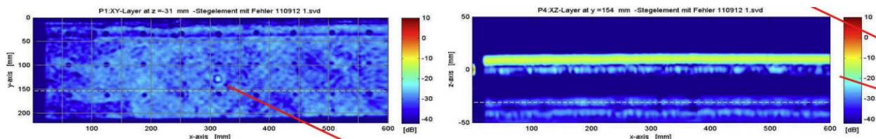
Figure 13. D-scan of GFRP component: wetting error (left), B-scan in profile line (right) (Becker, 2020).
