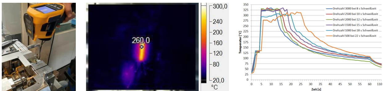
Figure 15. Passive thermography on friction welding of wooden bars (left), temperature plots for several speeds (right).
