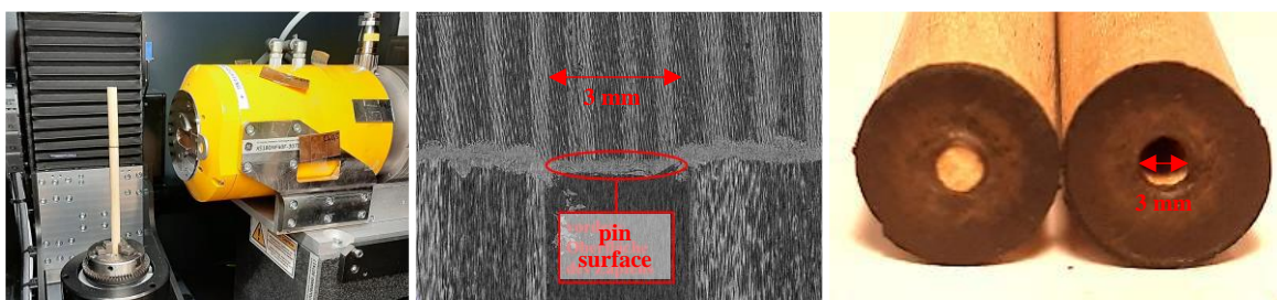
Figure 9. Pine sample in CT system (left), CT image (middle) and sample after tensile test (right).
