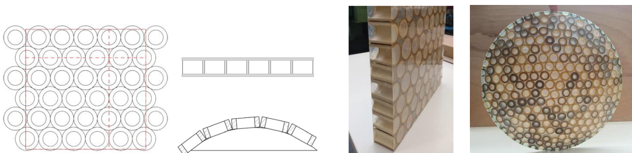
Figure 5. Comboo structure with GFRP top layer, potential for round structures “bamboo design” (Loth, 2019).
