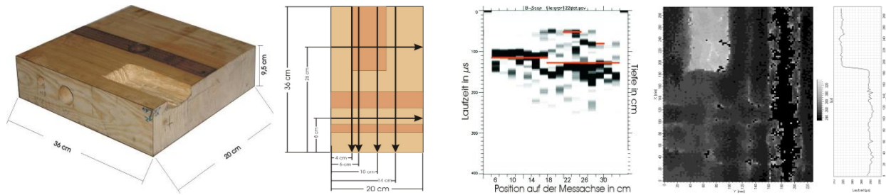
Figure 11. Test sample with dimensions (left), B-scan with echo technique (middle), C-scan non-contact measured in transmission (right) (Hasenstab, 2005).
