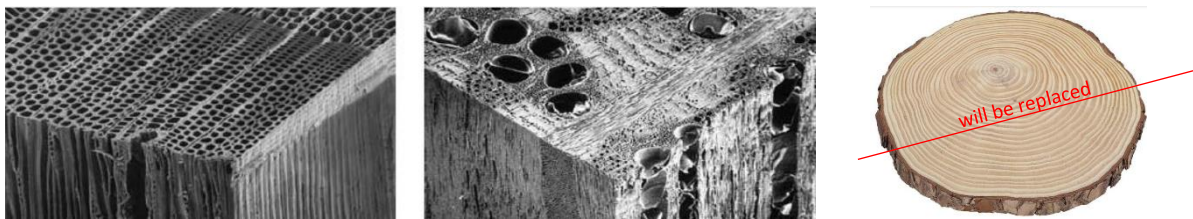
Figure 1. Inner structure of softwood (left), hardwood (middle) (Bühler, 2008), tree slice with annual rings (right).
