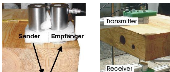
Figure 10. Ultrasonic puls-echo technique (left) and non-contact transmission mode (right) (Hasenstab, 2005).
