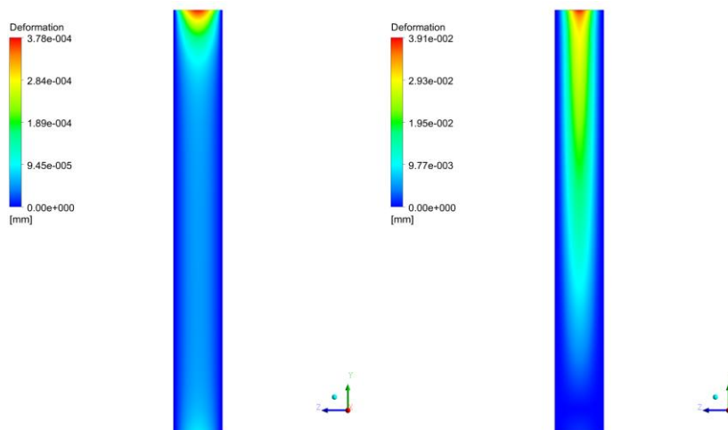
Figure 9. Total plate deformation for v_0 = 21.44 m/s with equal (left) and different (right) coolant channels.
