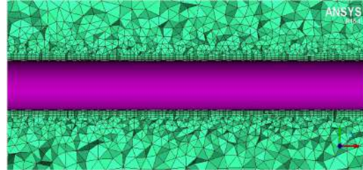
Figure 4: Boundary layer.
