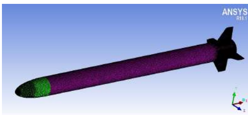
Figure 5: Rocket's mesh.
