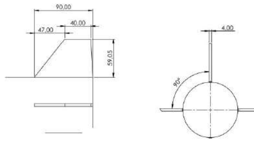
Figure 2: Fin's dimensions.
