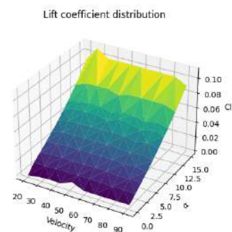
Figure 10: Lift Coefficient Distribution.
