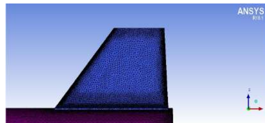
Figure 6: Fin's mesh.
