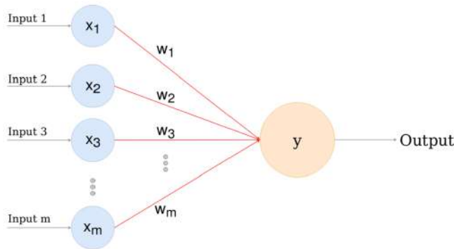
Figure 7: The Perceptron.
