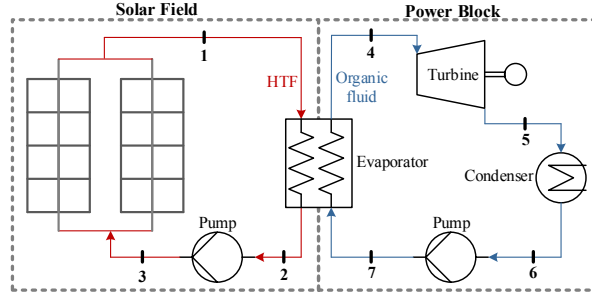
Figure 1. Schematic of SORC power system.
