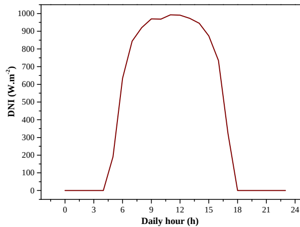
Figure 3. Daily DNI used in the simulation.
