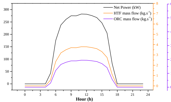
Figure 9. Net power, HTF and ORC mass flow rates under DNI variation.
