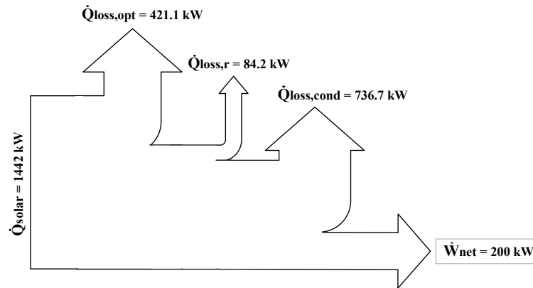
Figure 6. Sankey diagram of the system.
