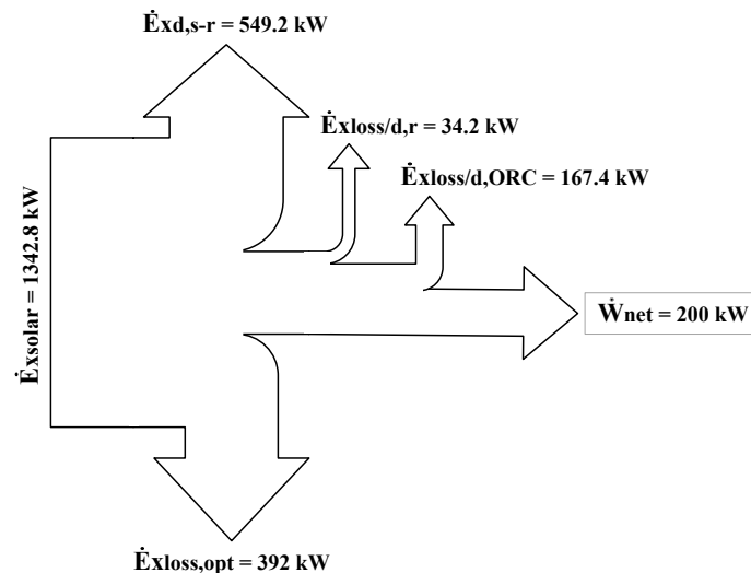
Figure 7. Grassmann diagram of the system.
