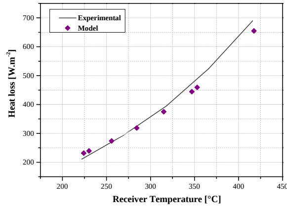
Figure 4. Solar field model validation.
