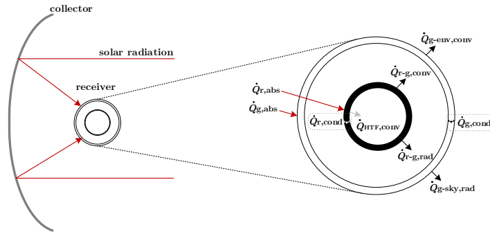
Figure 2. Heat transfer mechanisms in the cross-section receiver tube.
