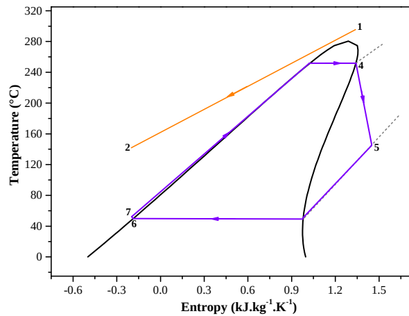
Figure 5. T - s diagram of the system.
