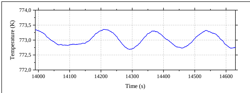
Figure 1. Preliminary heating test for 773 K set point, with 600 seconds temperature cutout.
