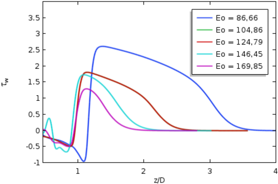
Figure 6: Wall shear stress in the axial direction in a fixed frame of reference bellow the bubble wake ( \tau_w ) of for distinct values of Eo Araújo et al. (2012).
