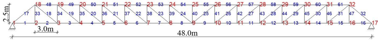
Figure 3 – Pratt truss footbridge proposed by Miguel et al. (2015)
