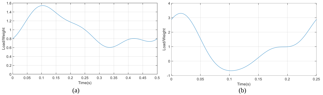
Figure 1 – Representation of the load function for a single person (a) walking and (b) running
