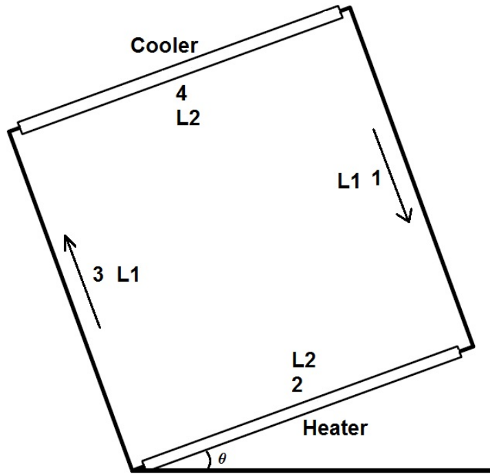
Figure 1. Natural circulation loop
