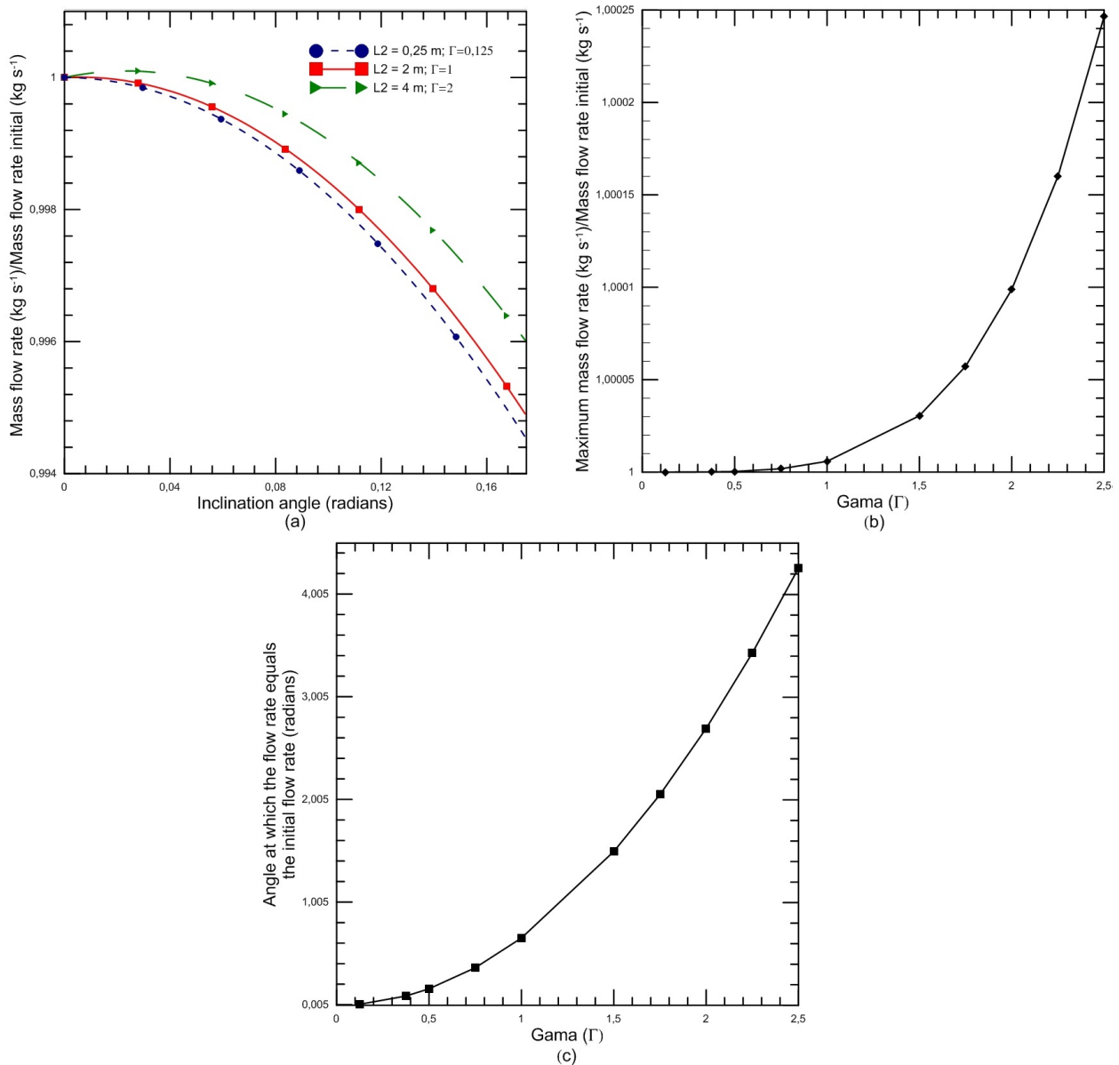
Figure 2. (a) Relative mass flow rate as function of the inclination angle ranges from 0° to 10°, (b) Relative mass flow rate maximum as function of \Gamma and (c) Angle at which the flow rate equals the initial flow rate as function of \Gamma .
