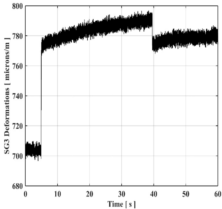
Figure 9. SG3 Signal transient from 14,0 to 14,5 m/s
