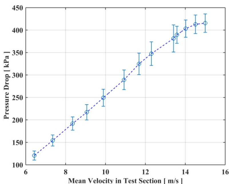
Figure 5. Pressure drop in the Test Section
