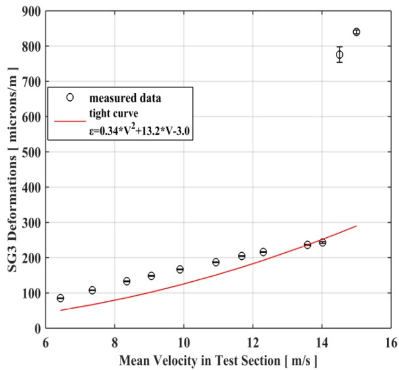
Figure 8. Deformations in the middle (SG3) of the Test Section
