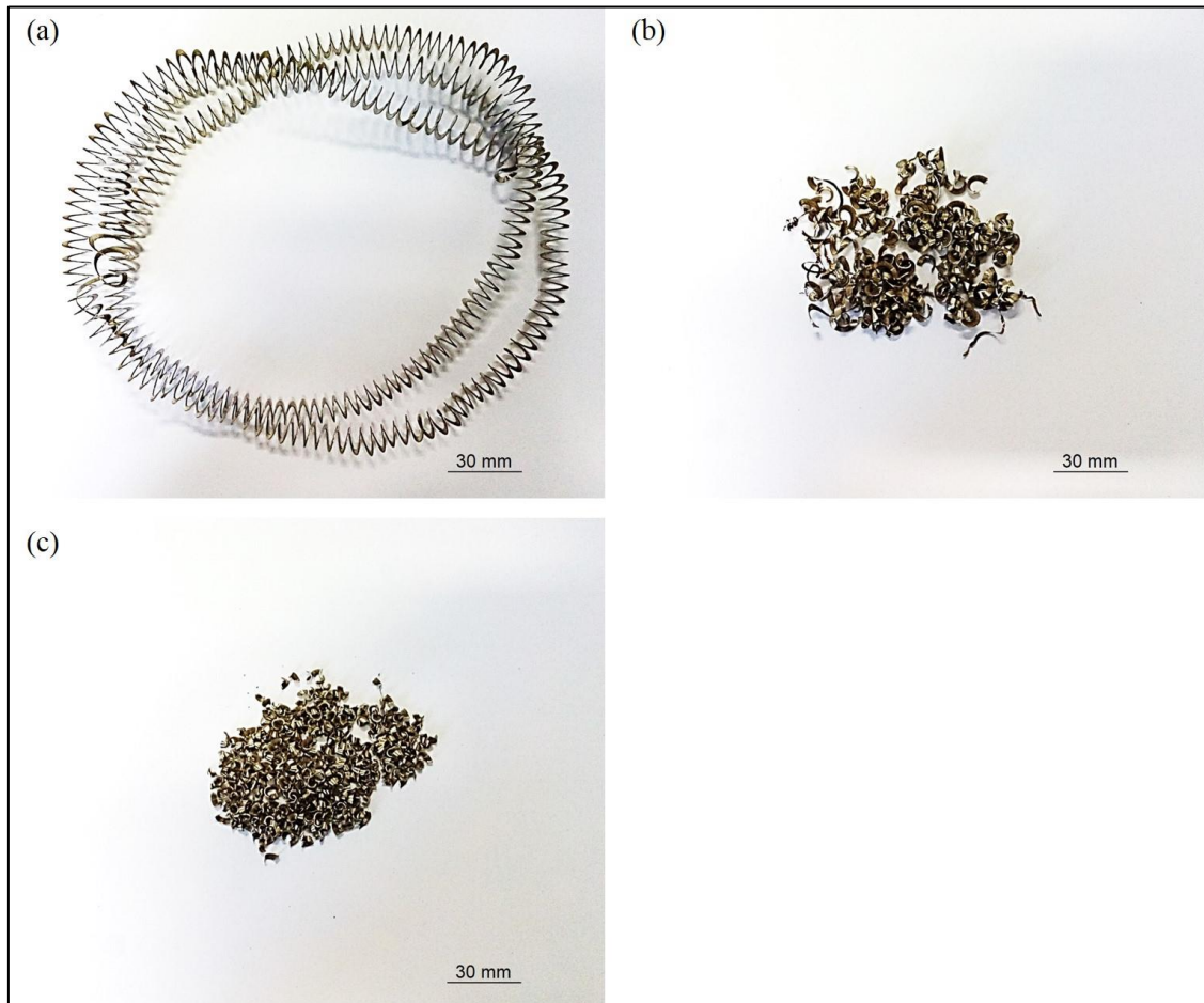
Figure 2. Chip forms. (a) Washer-type helical chip (reference tool); (b) Arc chip (chip-breaker model A); (c) Arc chip shorter than previously (chip-breaker model B)
